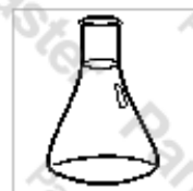
Flask 2
