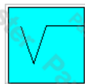
Square root
