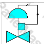
Diaphragm actuated valve with positioner
