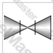
3-D Restriction orifice drilled in valve
