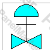
Valve, fail indeterminate
