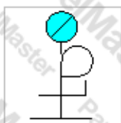
Pressure gauge with pigtail steam siphon
