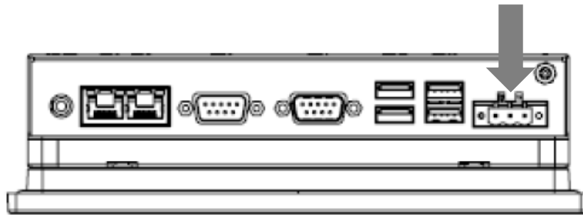
Figure 2.2 Power Connector
