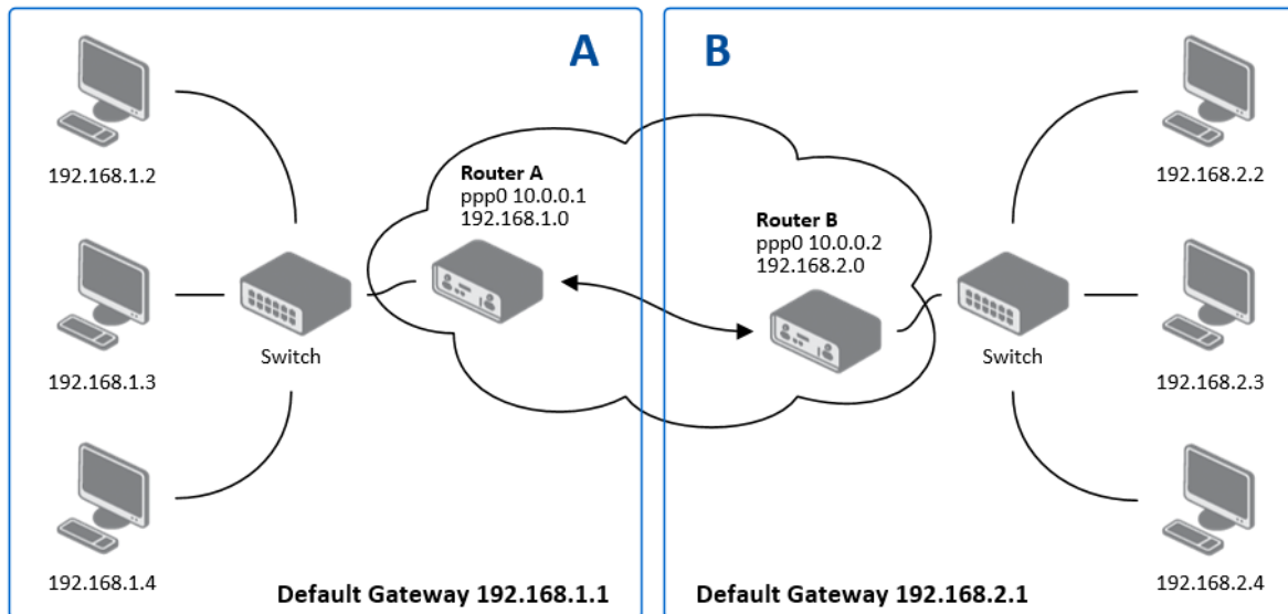
Figure 55: Topology of IPsec Configuration Example
